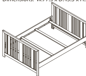
Imperia Bed Conversion Rails – 4916 Dimensions: W:54 x D:76 x H:35
